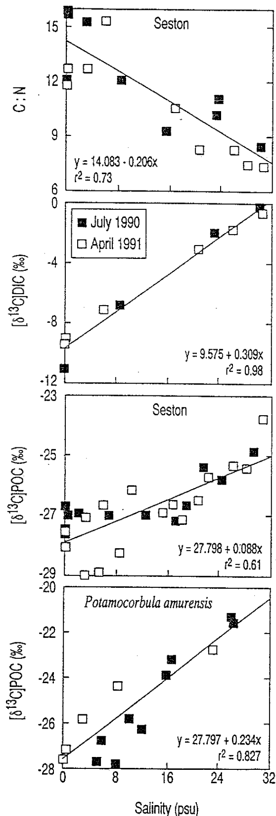
Fig. 4. Significant correlation ( P < 0.05 ) with salinity was found for several parameters measured along the salinity gradient in the NB. Data are presented for baseline (July 1990) and flood (April 1991) conditions.
