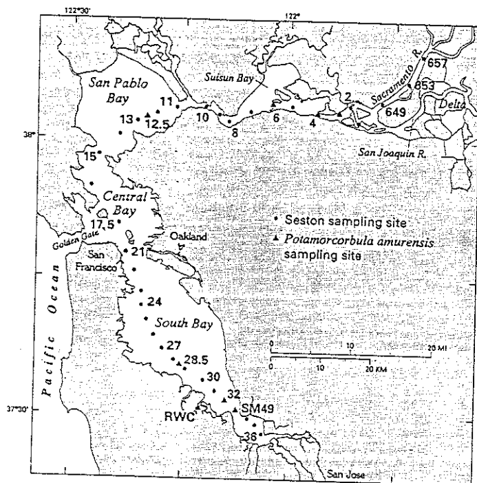
Fig. 1. Map of San Francisco Bay indicating sites where seston and P. amurensis samples were collected. The bay is divided into northern and southern regions by the Golden Gate. The northern region (NB) includes the lower Sacramento River (to Sta. 657), Suisun Bay, and San Pablo Bay; South Bay (SB) is the region to the south of the Golden Gate.
