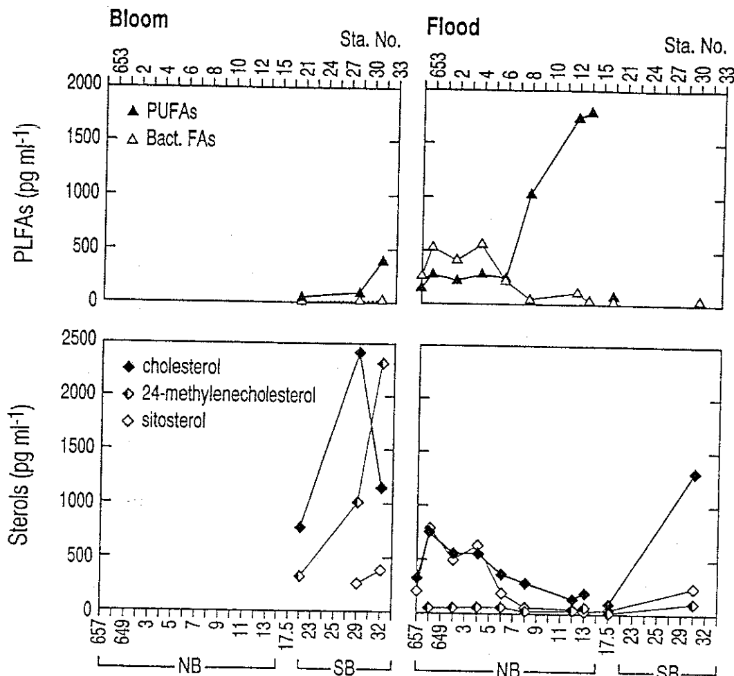
Fig. 6. Source-specific lipid compounds (PUFAs and bacterial fatty acids; sterols) associated with seston compared for two events thought to influence the origin of organic matter: the spring bloom and winter floods. PUFAs indicative of phytoplankton are compared with fatty acids specific to gram-positive bacteria (iso- and anteiso- C_{13} , C_{15} , and C_{17} ). PUFAs increased during the spring bloom in the SB as well as during a small bloom in SPB (Sta. 12, 13) that coincided with our "flood" cruise. Bacterial fatty acids (possibly associated with soils) were enriched at the freshwater end-member (Sta. 657-4) during periods of flow. The abundance of three sterols—cholesterol (ubiquitous), 24-methylenecholesterol (phytoplankton), and sitosterol (vascular plants, occasionally phytoplankton)—are compared in the lower panels.
