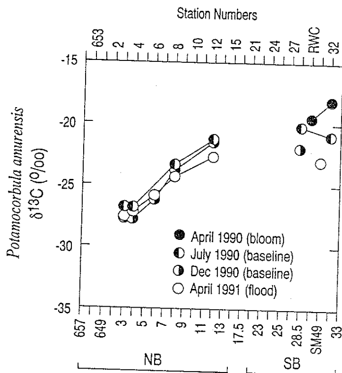
Fig. 5. Isotopic composition of P. amurensis collected on four dates. Values of [\delta^{13}\text{C}]\text{POC} in the clam tissues increased consistently from NB to SB. The heaviest values were measured in the SB (Sta. 32) during the spring bloom.
