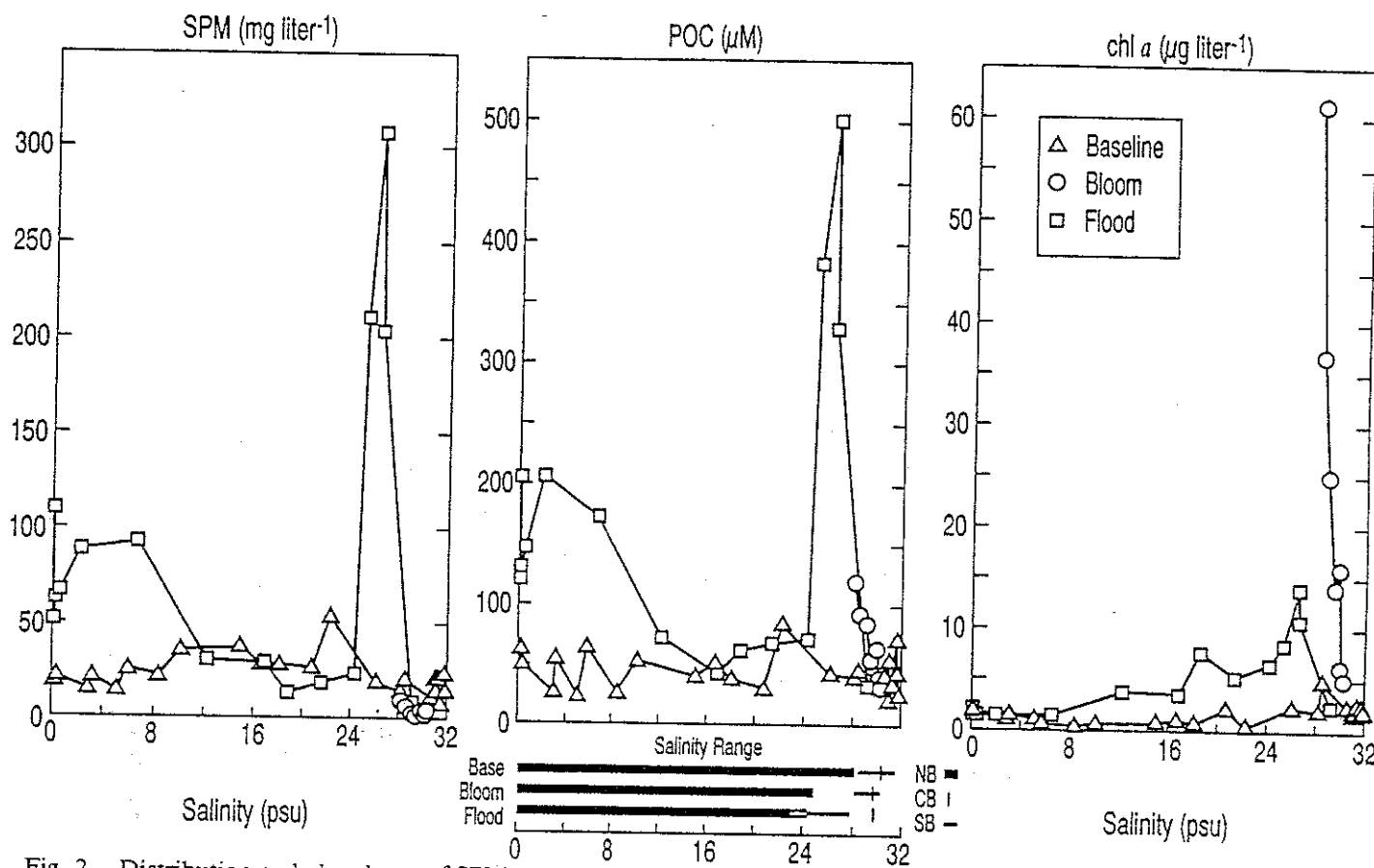
Fig. 2. Distribution and abundance of SPM, POC, and Chl a associated with seston. Samples were collected under three sets of conditions: the spring phytoplankton bloom in the SB (April 1990); winter storms, which include periods of freshwater inflow in the NB and wind-driven resuspension in the SB (March and April 1991); and baseline conditions (January, July, and December 1990). The data have been averaged in cases where there were multiple cruises. Salinity ranges for each sampling condition (baseline, bloom, and flood) are provided below the center panel (CB—the central bay).
